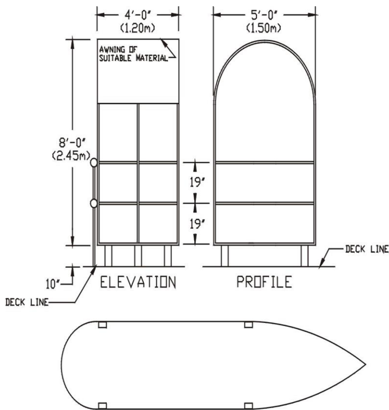
FIGURE 2 – Pilot Platforms
